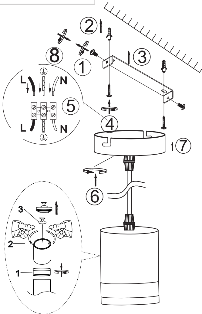
The step to change bulb
